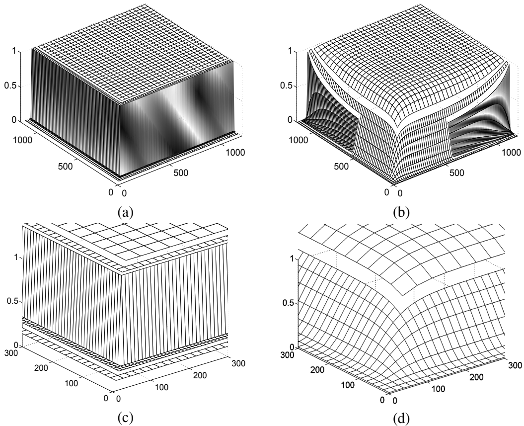
FIGURE 4. Cash-or-Nothing option: (a) The initial configuration at time \tau = 0 . (b) The final configuration at time \tau = 1 . (c) and (d): Magnified representations of (a) and (b), respectively.
