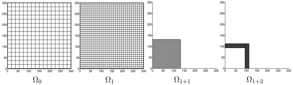
FIGURE 1. Hierarchy of grids when l = 1 and l^* = 2 .
