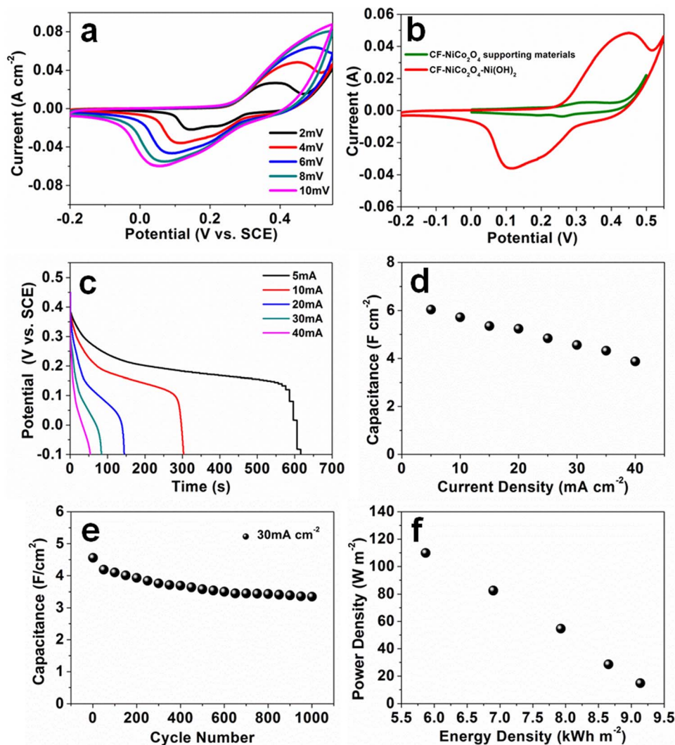
Figure 4 | Electrochemical characterizations of the 3D hybrid nanostructured CF-NiCo 2 O 4 -Ni(OH) 2 electrode. (a) CV curves at various scanning rates from 2 to 10 mV S -1 ; (b) CV curves comparison of the CF-NiCo 2 O 4 supporting materials and CF-NiCo 2 O 4 -Ni(OH) 2 electrode at scanning rate of 4 mV s -1 (c) Discharge voltage profiles at various current densities from 5 to 40 mA cm -2 ; (d) The change in capacitance with increasing current density; (e) The capacitance cycling performance at a constant current density of 30 mA cm -2 ; (f) Areal energy density and areal power density of CF-NiCo 2 O 4 -Ni(OH) 2 electrode evaluated at different current density.
