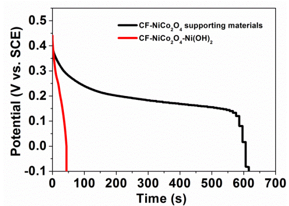
Fig. S1. The discharging curves of the CF-NiCo 2 O 4 supporting materials and the CF-NiCo 2 O 4 -Ni(OH) 2 electrode at the current density of 5 mA cm -2
