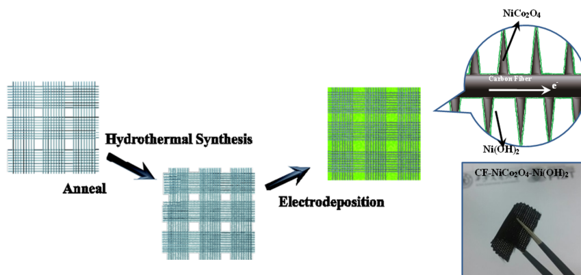
Figure 1 | Schematic diagram of the preparation procedure of the CF-NiCo 2 O 4 -Ni(OH) 2 3D hybrid structured electrode material.
