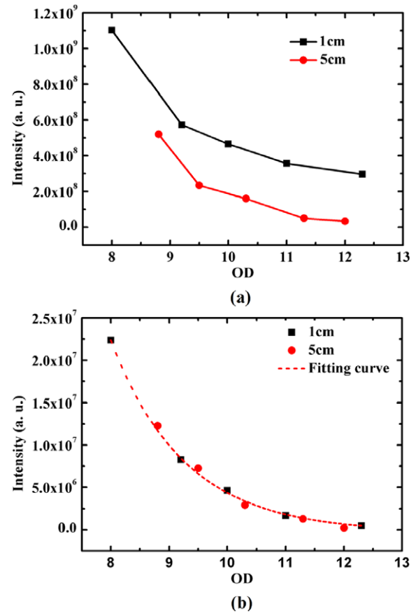
Figure 6. Image intensities for the 1 and 5 cm-thick suspensions of 0.7 μm polystyrene microspheres at different ODs. (a) Direct imaging. (b) Optical Kerr gated imaging.
