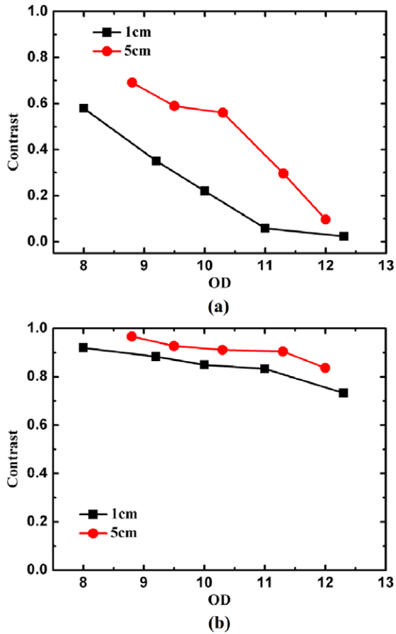
Figure 5. Image contrasts for the 1 and 5 cm-thick suspensions of 0.7 μm polystyrene microspheres at different ODs. (a) Direct imaging. (b) Optical Kerr gated imaging.
