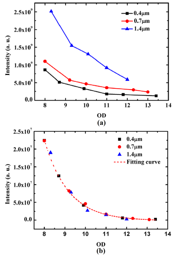
Figure 4. Image intensities for the suspensions of 0.4, 0.7 and 1.4 \mu\text{m} polystyrene microspheres at different ODs. (a) Direct imaging. (b) Optical Kerr gated imaging.
