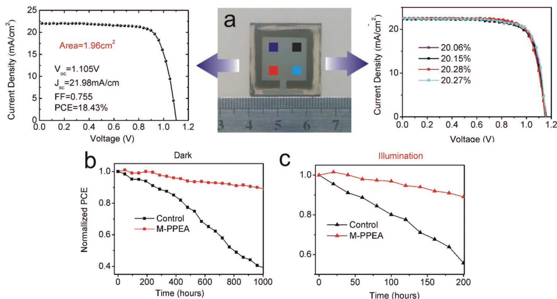
Figure 7. a) J - V curves measurements of large area ( 1.96 \text{ cm}^2 ) and small region devices ( 0.09 \text{ cm}^2 ); b) dark stability and c) working stability (1 sun illumination) of the devices with pristine and M-PPEA films.
