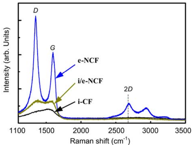
Fig. 4 Raman spectra of the carbon films with different irradiation methods.
