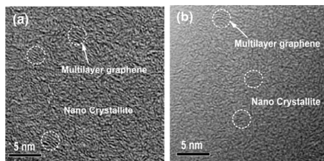
Fig. 7 TEM images at low frictional wear tracks of (a) e-NCF, and (b) i-CF.
