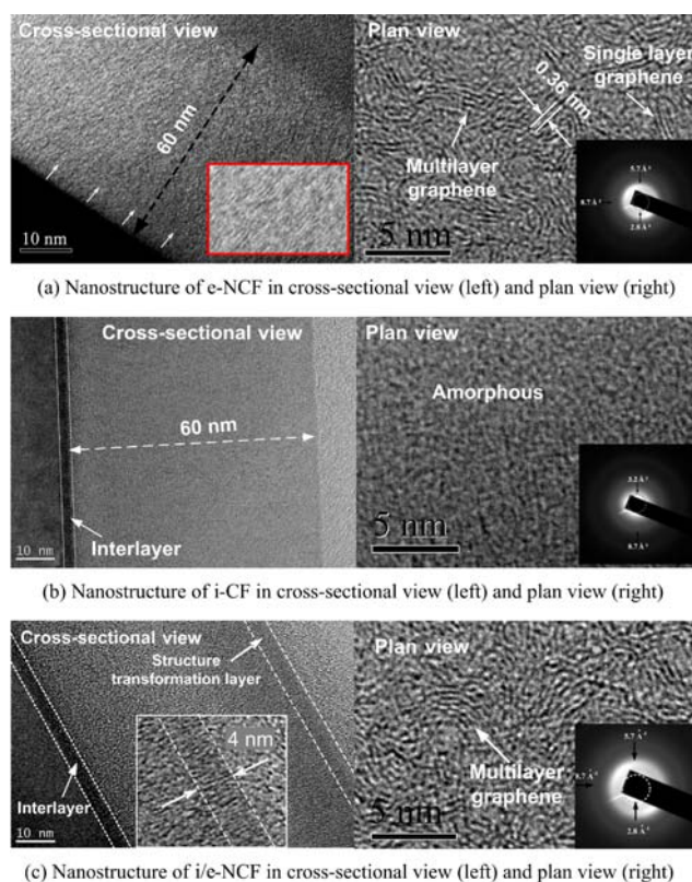
Fig. 3 TEM images of the carbon films with different irradiation methods.
