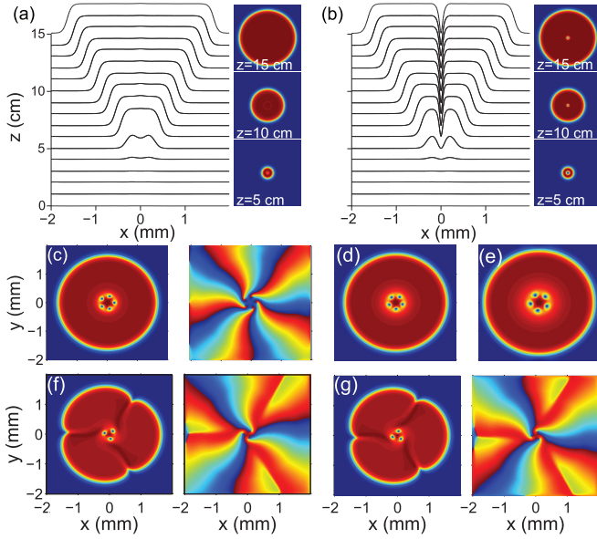
FIG. 2. (Color online) (a) and (b) Evolution of vortex incidences during propagation for l = 0 and 1 , respectively. The right panels are selected intensities when the beam propagates to z = 5 , 10 , and 15 cm, respectively. (c) Intensities and phases of vortices with l = 5 at z = 15 cm. In (a)–(c) \beta = 0.5 . (d) and (e) Intensities of vortices with l = 5 at z = 15 cm when \beta = 1 and \beta = 2 , respectively. (f) and (g) Intensities and phases of trilobe inputs ( n = 1.5 ) at z = 15 cm corresponding to l = -4.5 and 4.5 , respectively.
