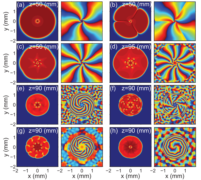
FIG. 6. (Color online) Intensities and phases of (a) a vortex with l = 5 , n = 0 , (b) a necklace with l = 4.5 , n = 1.5 , and (c) an azimuthon with l = 6 , n = 3 , for r_0 = 100 \mu\text{m} , respectively. (d)–(f) Azimuthons with l = 9 , n = 3 , for r_0 = 40 , 20 , and 23 \mu\text{m} , respectively. (g) and (h) Azimuthons with r_0 = 20 \mu\text{m} , n = 4 , for l = 4 and l = 6 , respectively.
