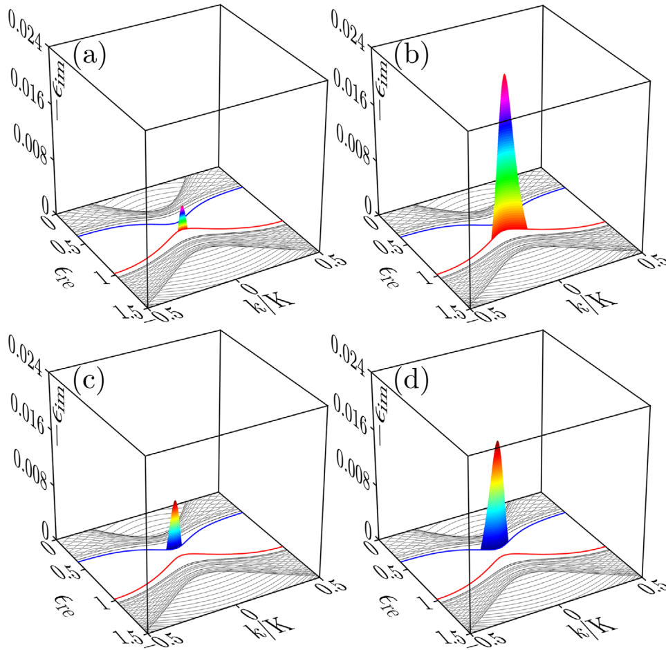
Figure 2. Real \epsilon_{re} and imaginary \epsilon_{im} parts of energy of the linear VESs. (Top) Type-I gain landscape on the armchair domain wall, a) p_{im} = 0.3 and b) p_{im} = 0.4 . (Bottom) Type-II gain landscape, c) p_{im} = 0.35 and d) p_{im} = 0.4 . Only states with -\epsilon_{im} > 0 can lase, while all other states are attenuated.
