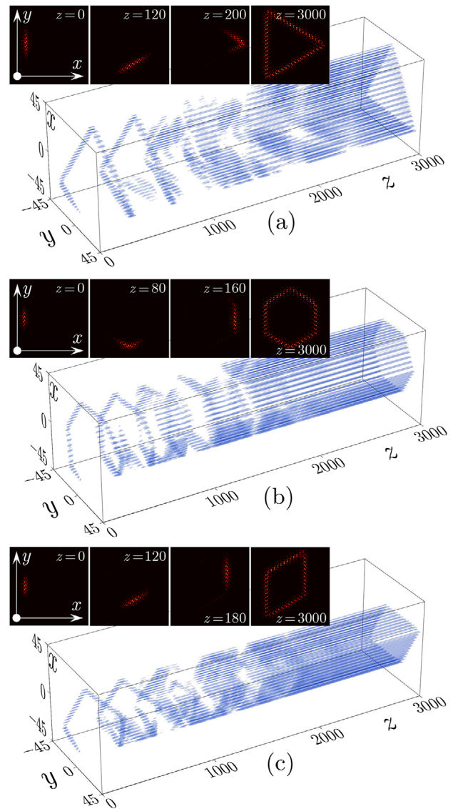
Figure 6. Examples of topological lasing patterns with moving VHESs in different geometries. Circulation of the VHESs and transition to stable lasing in a) triangular, b) hexagonal, and c) rhombic structures at \gamma = 0.005 , p_{\text{im}} = 0.045 and \alpha = 0.3 . The initial state corresponds to the linear edge state with momentum k = 0.1K with superimposed envelope of the width w = 9b .
