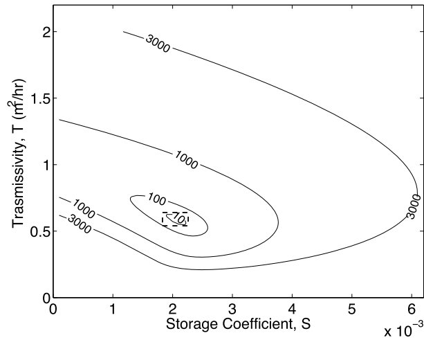
Figure 9.2 \chi^2 contour plot for the slug test for a wide range of parameters. The small box shows the close-up axis range displayed in Fig. 9.3.
