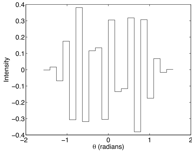
Figure 3.19 \mathbf{V}_{:,18} for the Shaw example problem.
