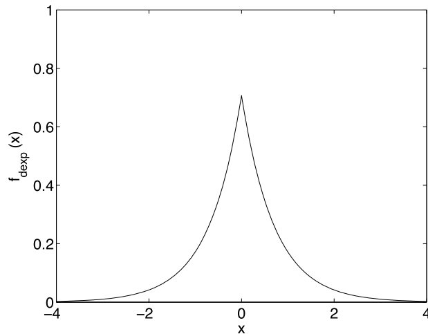
Figure B.6 The double-sided exponential probability density function ( \mu = 0, \sigma = 1 ).
