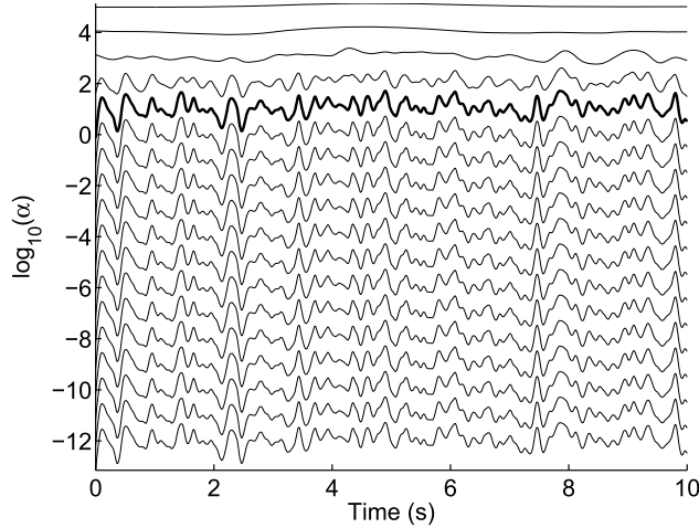
Figure 7.13 Signal recovery obtained using second-order Tikhonov regularization. Solution amplitudes are normalized to improve legibility.
