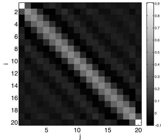
Figure 4.8 Resolution matrix for the Shaw problem, \alpha = 4.29 \times 10^{-5} . Note that the noise-free inversion of a spike model e_j will produce the i th column or row of \mathbf{R}_m (e.g., Fig. 4.7 is a plot of the 10th column/row).
