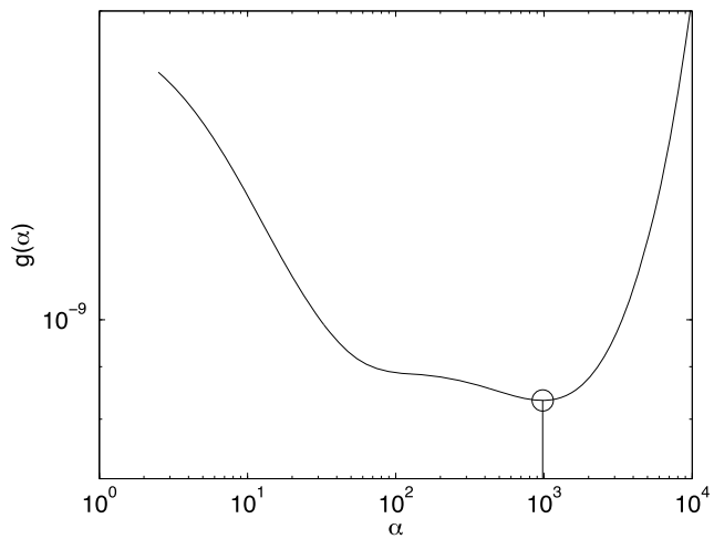
Figure 4.23 GCV curve for the VSP problem and its minimum, second-order regularization.
