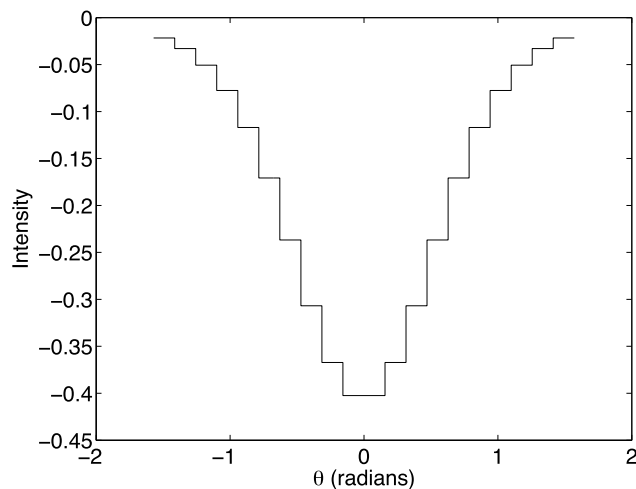
Figure 3.20 V_{:,1} for the Shaw example problem.
