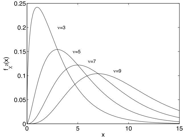
Figure B.4 The \chi^2 probability density function for several values of \nu .
