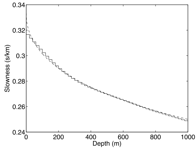
Figure 4.25 GCV solution for the VSP problem, second-order, \alpha = 981 , shown in comparison with the true model.
