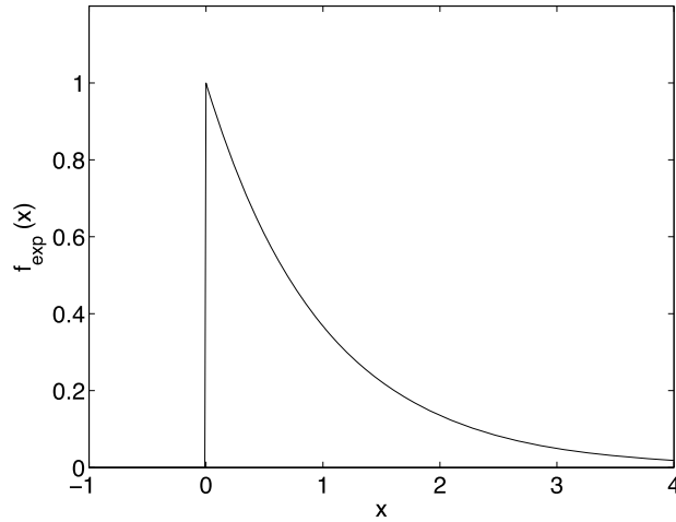
Figure B.5 The exponential probability density function ( \lambda = 1 ).
