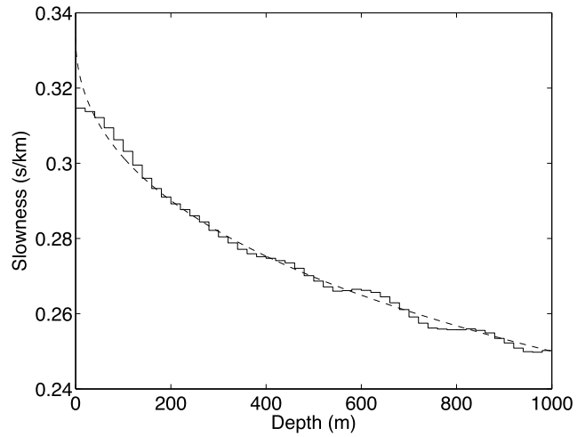
Figure 4.24 GCV solution for the VSP problem, first-order, \alpha = 76.3 , shown in comparison with the true model.
