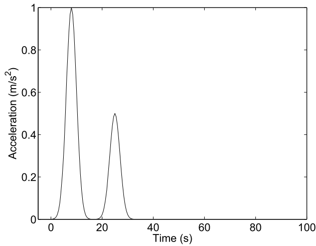
Figure 3.13 Generalized inverse solution using all 210 singular values for the noise-free data.
