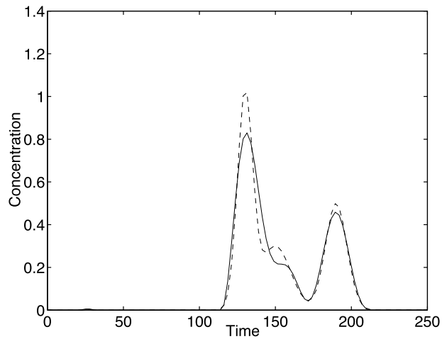
Figure 4.34 Second-order Tikhonov regularization source history solution determined from the L-curve of Fig. 4.33, with true history (Fig. 4.28) shown as a dashed curve.
