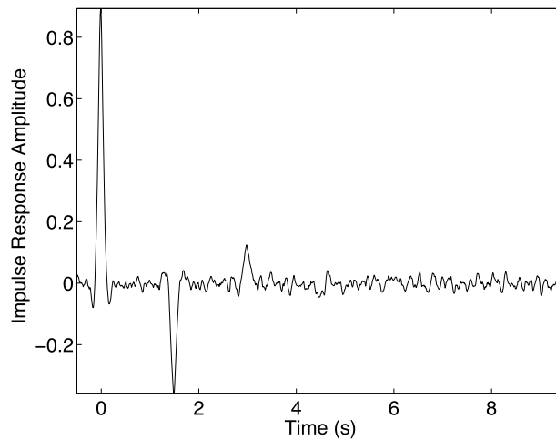
Figure 7.6 Zeroth-order Tikhonov solution.
