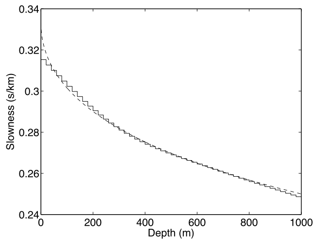
Figure 4.15 Tikhonov solution for the VSP problem, second-order regularization, \alpha = 2341 , shown in comparison with the true model (Fig. 4.10).
