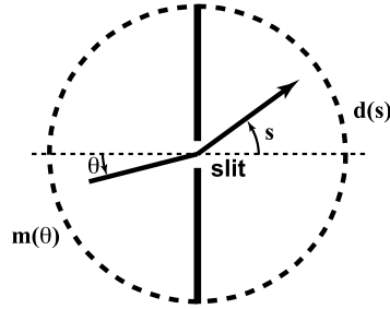
Figure 1.6 The Shaw diffraction intensity problem (1.26), with model and data represented as functions of angles \theta and s .
