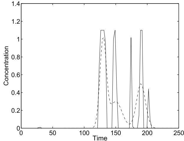
Figure 4.32 BVLS source history solution ( l = 0, u = 1.1 ) with true history (Fig. 4.28) shown as a dashed curve.
