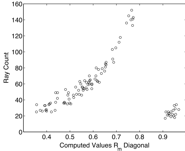
Figure 6.15 Comparison of ray densities and resolution.
