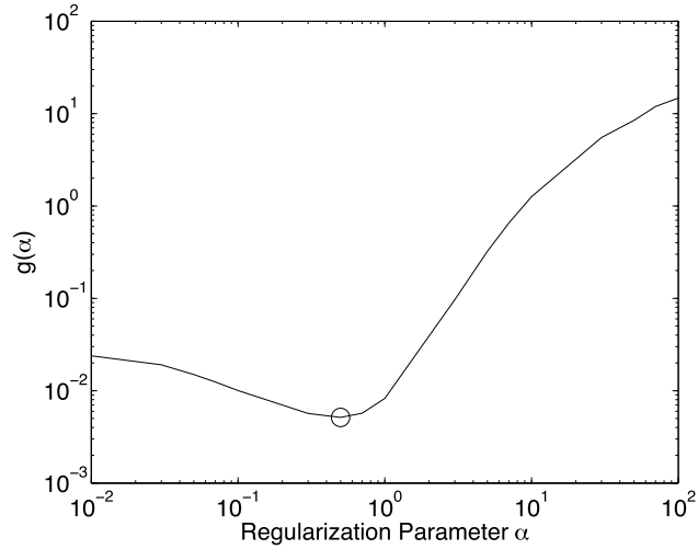
Figure 6.13 GCV plot for the tomography example of Fig. 6.11 and its minimum near \alpha = 0.5 .
