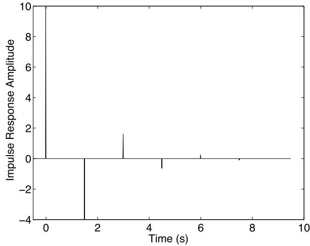
Figure 7.3 The true impulse response model m(t) .
