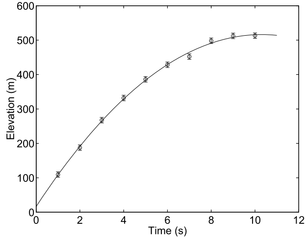
Figure 2.1 Data and model predictions for the ballistics example, with 1 standard deviation data error bounds indicated.
