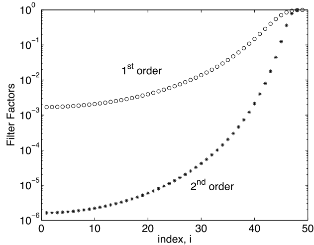
Figure 4.16 Filter factors (4.17) for optimal first- and second-order Tikhonov solutions to the VSP problem shown in Figs. 4.13 and 4.15.
