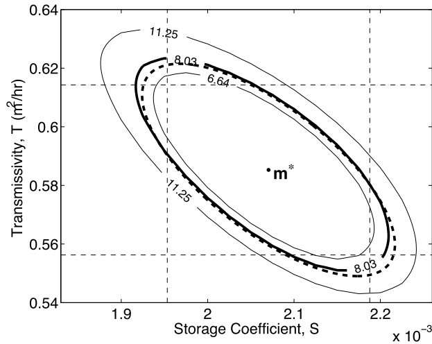
Figure 9.3 Closeup \chi^2 contour plot for the immediate vicinity of the optimal parameters \mathbf{m}^* for the slug test example, showing nonlinear 90%, 95% (bold) and 99% confidence contours. The nearly elliptical contours are indicative of an approximately linear behavior at this scale. Dashed ellipse shows the linearized approximation to the 95% confidence contour calculated using (9.38). 95% confidence intervals for the parameters calculated from (9.38) are shown as dashed lines.
