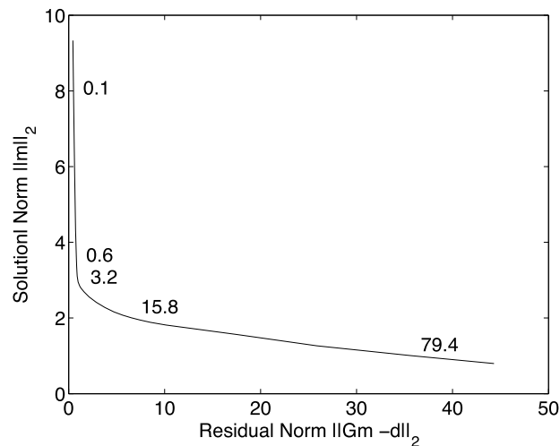
Figure 8.4 L-curve for a logarithmically distributed range of water level values, as indicated.
