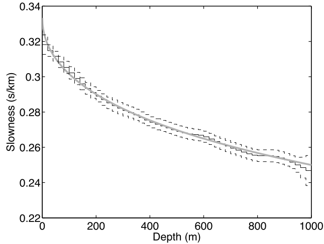
Figure 11.13 MAP model obtained from the posterior distribution, and its 95% distribution intervals, using the prior distribution depicted in Figs. 11.9 and 11.12. The true model is shown as the gray smooth curve.
