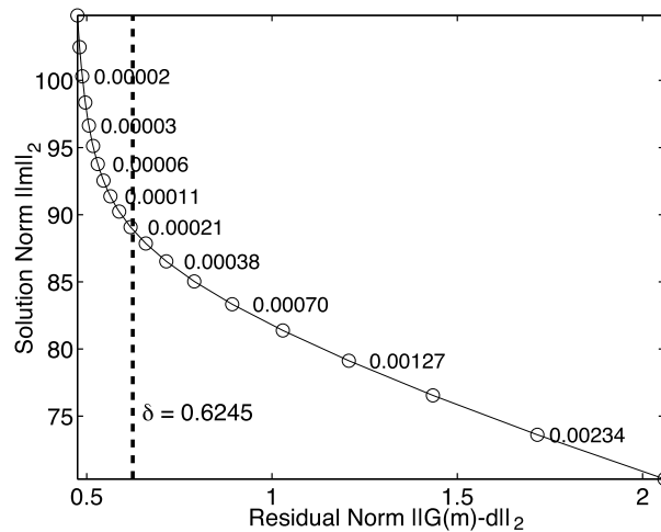
Figure 10.12 L-curve of solutions for the adjoint heat flow example, showing values of the Tikhonov regularization parameter and the discrepancy principle value of the residual norm.
