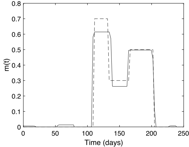
Figure 7.22 TV solution corresponding to the L-curve corner solution (Fig. 7.21) compared with the (sharp features) true model (dashed curve).
