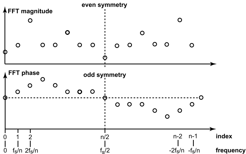
Figure 8.1 Frequency and index mapping for the DFT of a real-valued sequence ( n = 16 ) sampled at f_s . For DFT theory to accurately represent Fourier operations on a continuous time signal, f_s must be greater than or equal to the Nyquist frequency (8.36).
