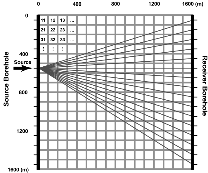
Figure 4.35 Cross-well tomography problem, showing block discretization, block numbering convention, and one set of straight source-receiver ray paths.
