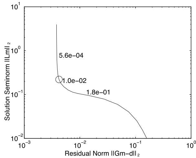
Figure 4.33 L-curve for the second-order Tikhonov solution with BVLS ( l = 0, u = 1.1 ) implementation, corner at \alpha = 0.01 .
