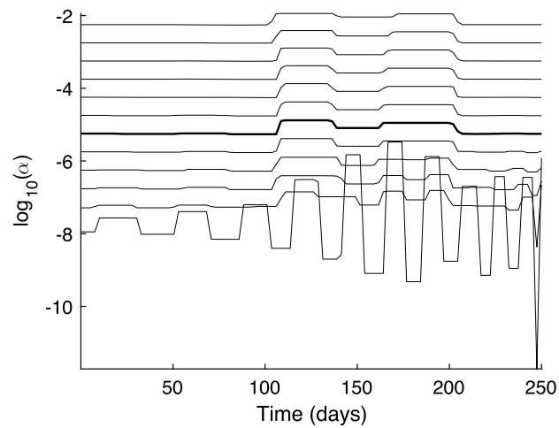
Figure 7.21 TV solutions for a range of \alpha values, with the solution for the corner at \alpha = 5.6 \times 10^{-6} (Fig. 7.20) shown in bold.
