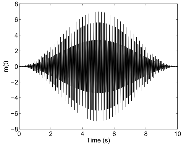
Figure 7.12 A 1001-point signal consisting of 25 and 35 Hz cosines (7.19), multiplied by a Hann taper.
