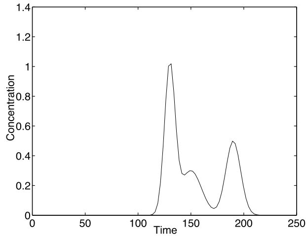
Figure 4.28 True source history.
