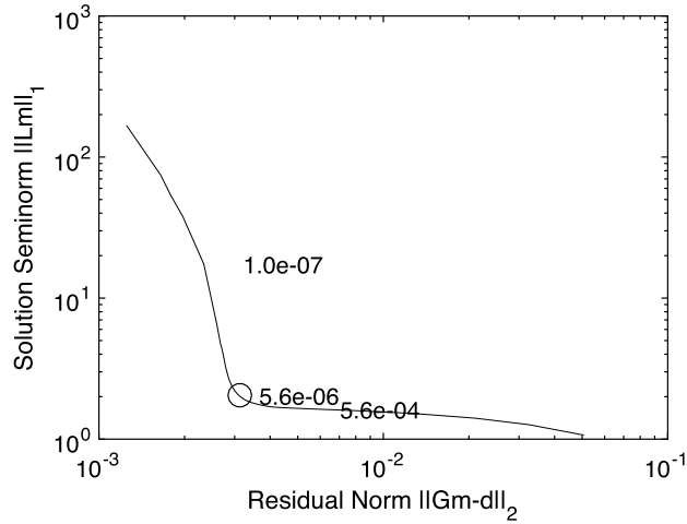
Figure 7.16 TV L-curve, with a corner at \alpha = 5.6 \times 10^{-6} .
