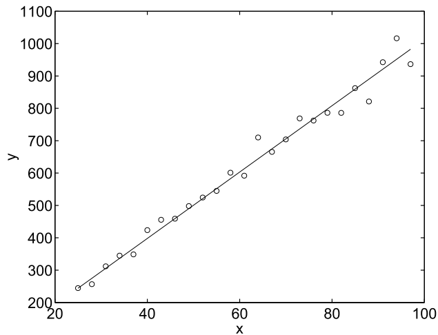
Figure 2.5 Data for Example 2.3, and corresponding linear regression line, weighted system.
