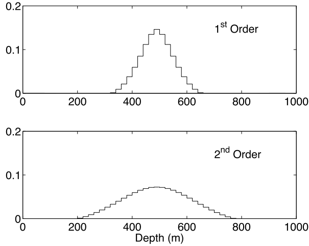
Figure 4.17 The model resolution matrix \mathbf{R}_{\alpha,L} multiplied times the spike model for the first- and second-order regularized solutions of Example 4.4.
