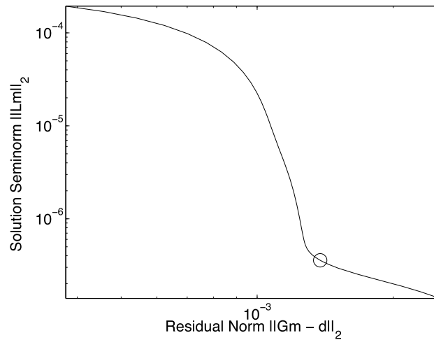
Figure 4.14 L-curve and corner for the VSP problem, second-order regularization.
