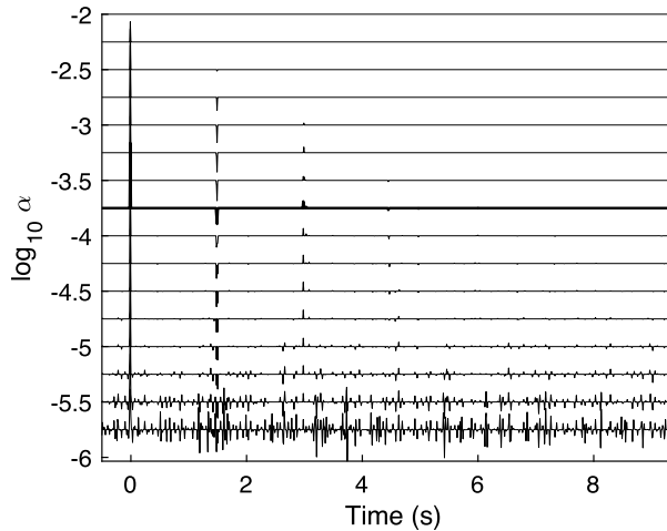
Figure 7.8 1-norm regularized solutions corresponding to the L-curve shown in Fig. 7.7. Model corresponding to the L-curve corner is shown in bold and is reproduced in Fig. 7.9.
