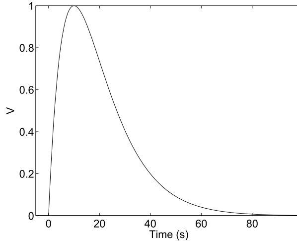
Figure 3.9 Example instrument response; output voltage in response to a unit area ground acceleration impulse (delta function).
