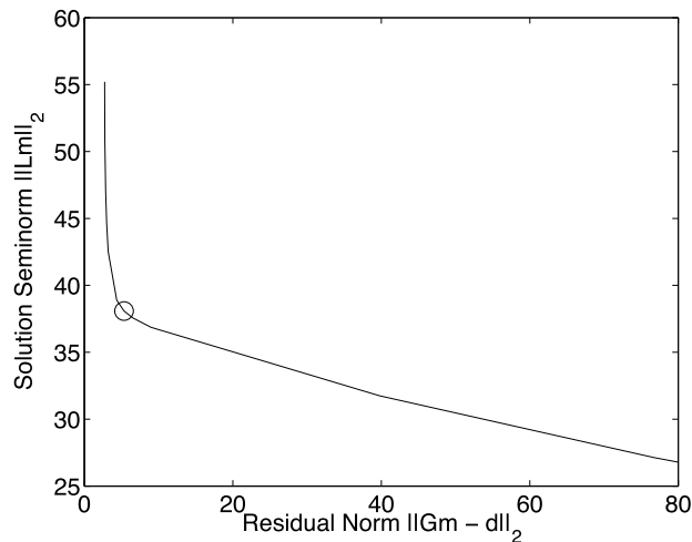
Figure 6.12 L-curve for the tomography example of Fig. 6.11 and its corner near \alpha = 0.5 .
