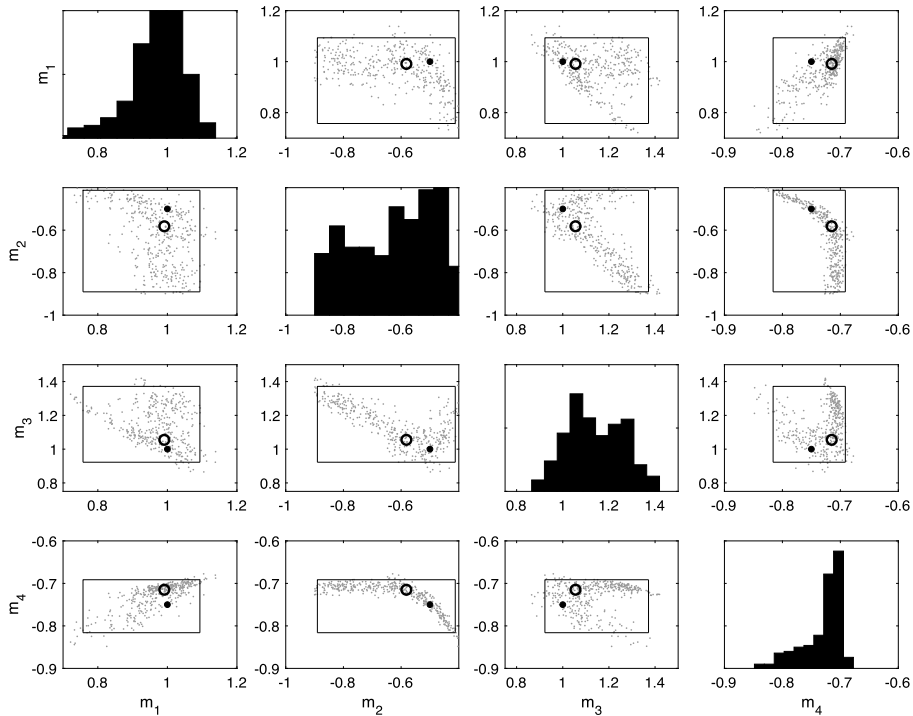
Figure 11.16 Sampled posterior distribution for Example 11.4. The true model is shown as the large black dot and the MAP model estimated from the maximum likelihood posterior distribution sample is indicated by the open circle. 400 retrieved samples of the posterior distribution (every 10,000th calculated sample from the MCMC output) are shown as gray dots. 95% probability intervals estimated from the MCMC posterior distribution samples are shown by boxes.
