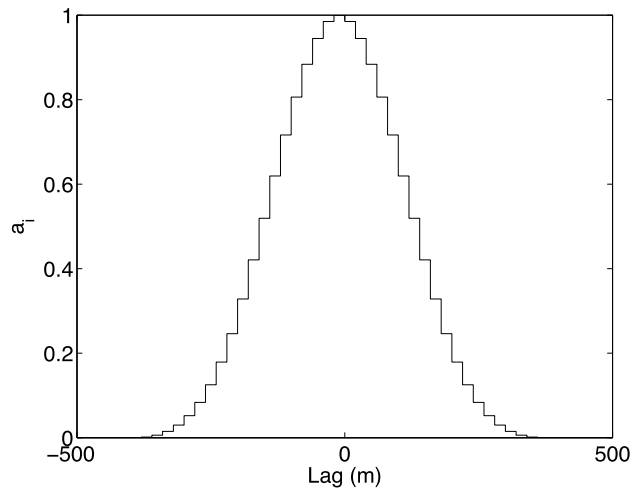
Figure 11.12 A correlation function for the prior distribution of Fig. 11.9 with a 1/e correlation length of approximately 10 parameters (200 m).
