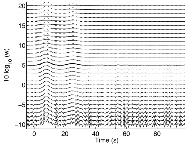
Figure 8.5 Models corresponding to the range of water level values used to construct Fig. 8.4. Dashed curves show the true model and bold trace shows the L-curve determined model with w = 3.16 (Fig. 8.4).
