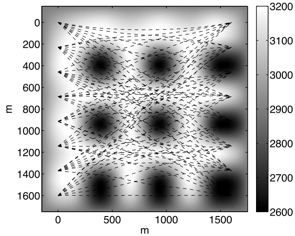
Figure 10.9 Checkerboard test model and ray paths for the cross well tomography problem of Example 10.1.
