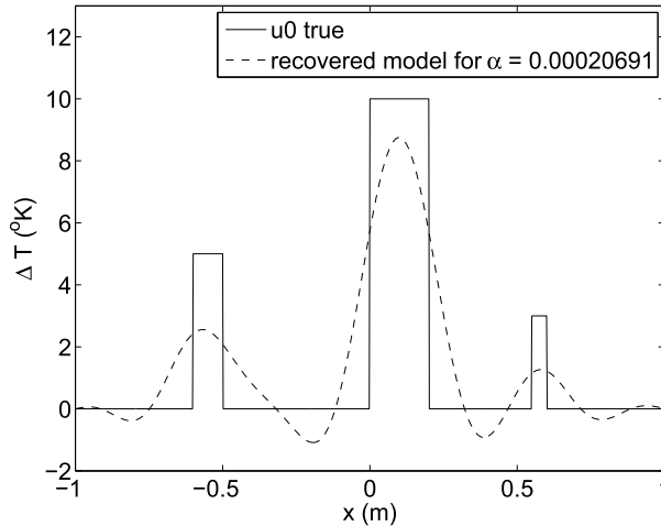
Figure 10.13 True initial condition and inverse solution with regularization parameter determined from the discrepancy principle as shown in Fig. 10.12.
