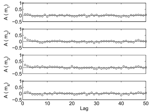
Figure 11.15 Autocorrelations for posterior distribution parameters (Fig. 11.17) after thinning to every 10,000th sample.
