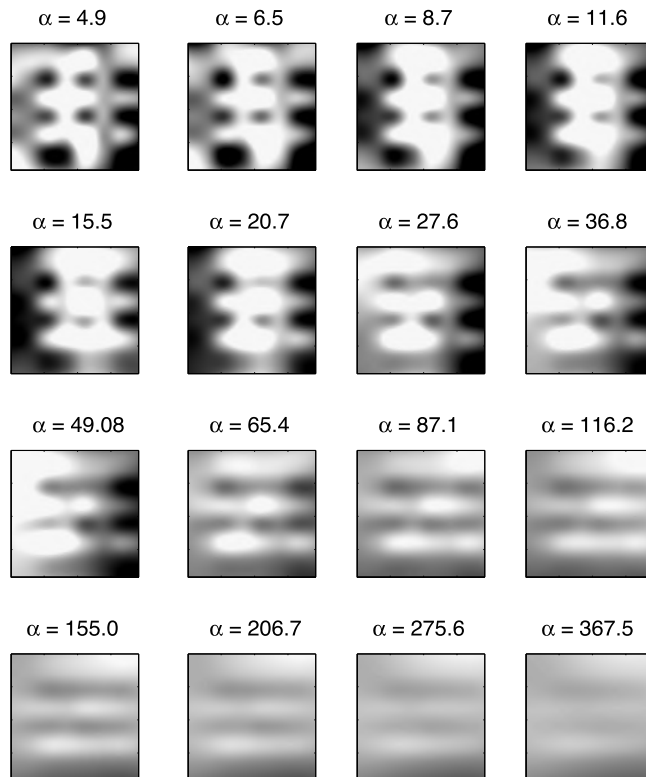
Figure 10.10 Suite of recovered models for a range of regularization parameter values (same as in Fig. 10.2) for the checkerboard test model of Fig. 10.9.
