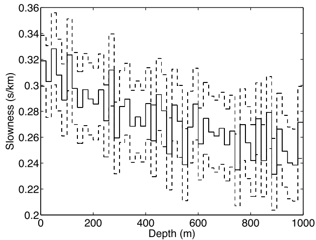
Figure 4.11 Least squares solution for the VSP problem, with 95% confidence intervals.
