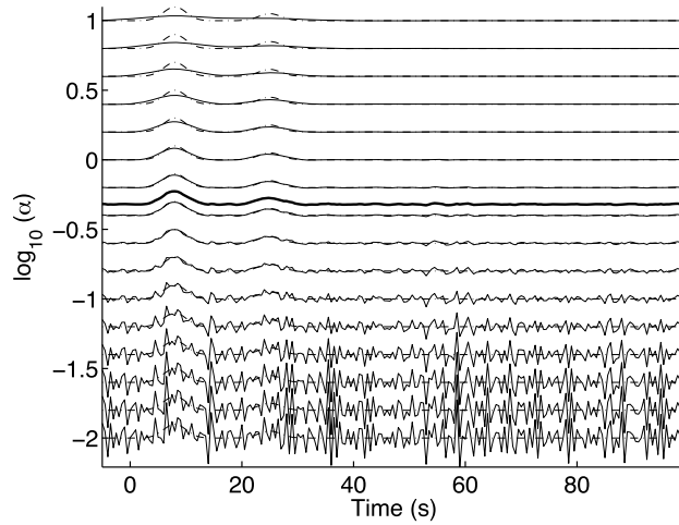
Figure 8.8 Zeroth-order Tikhonov regularized models corresponding to the range of regularization parameters used to construct Fig. 8.7. Dashed curves show the true model and bold trace shows the L-curve determined model with \alpha = 0.48 .
