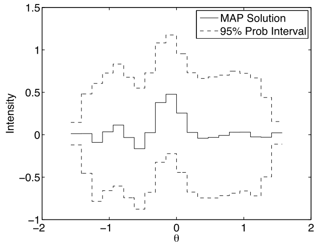
Figure 11.4 The MAP solution of Fig. 11.3, with 95% probability intervals.
