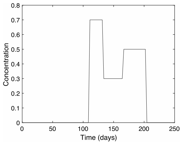
Figure 7.19 An alternative true source history for the source reconstruction problem with sharp features.
