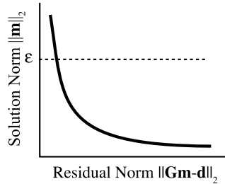
Figure 4.2 A particular model norm, \epsilon , and its position on the tradeoff curve between residual misfit, \|\mathbf{G}\mathbf{m} - \mathbf{d}\|_2 and model norm, \|\mathbf{m}\|_2 .
