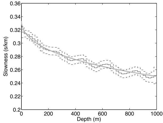
Figure 11.11 MAP model obtained from the posterior distribution, and its 95% distribution intervals, using the prior distribution described in Figs. 11.9 and 11.10. The true model is shown as the gray smooth curve.
