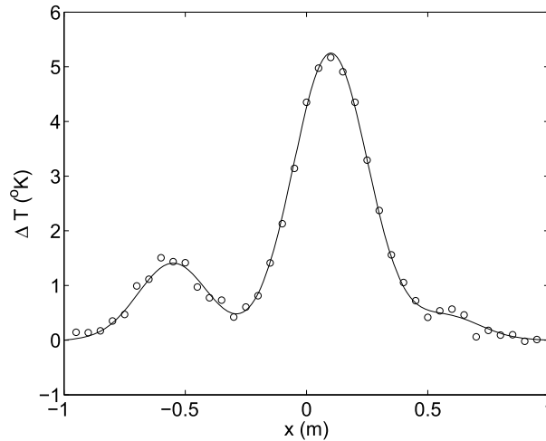
Figure 10.11 Temperature anomaly data at t = 10,000 s. The noise-free temperature anomaly is shown as a smooth curve.
