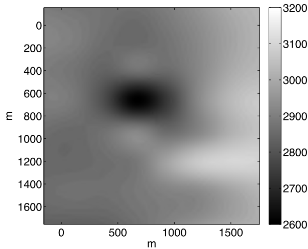
Figure 10.4 Best solution velocity structure (m/s), \alpha selected using the discrepancy principle, \alpha \approx 37 .
