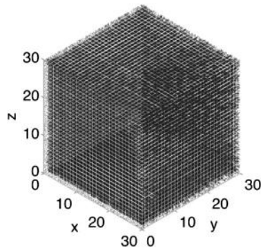
Figure 6.11 A 30 by 30 by 30 block tomography model interrogated by 30,000 ray paths.
