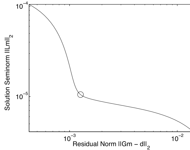
Figure 4.12 L-curve and corner for the VSP problem, first-order regularization.
