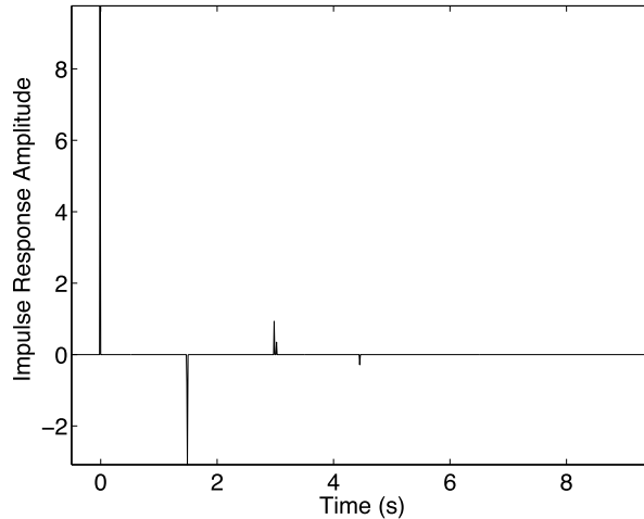
Figure 7.9 1-norm regularized solution for \alpha = 1.8 \times 10^{-4} (Fig. 7.8).
