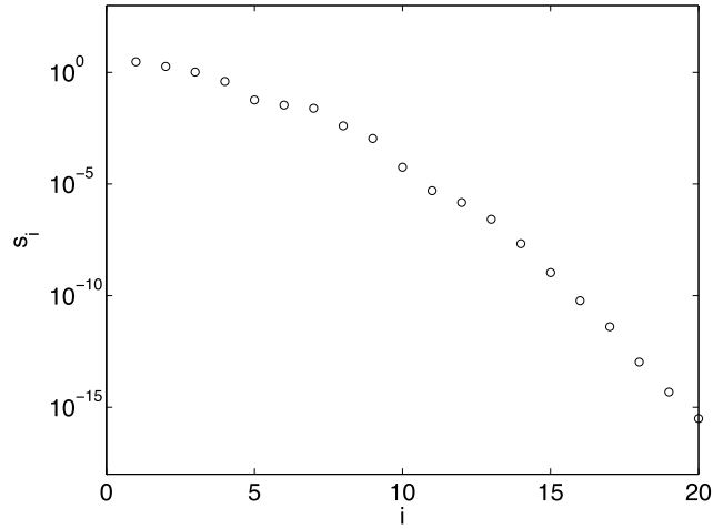
Figure 3.18 Singular values of \mathbf{G} for the Shaw example ( n = m = 20 ).
