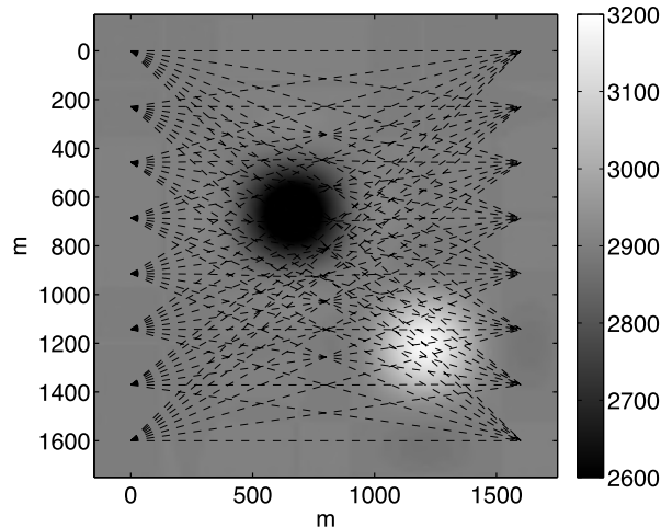
Figure 10.1 True velocity model and the corresponding ray paths for the bent-ray cross-well tomography example.
