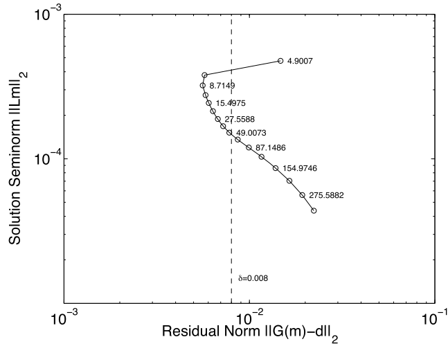
Figure 10.3 L-curve and corresponding \alpha values for the solutions of Fig. 10.2.
