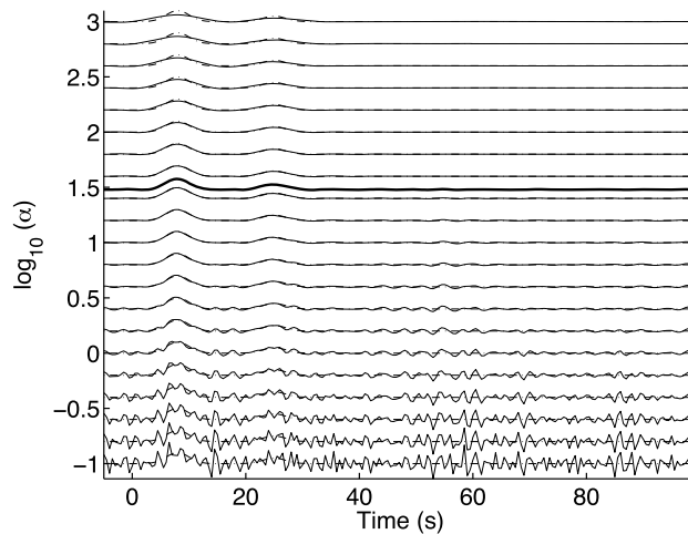
Figure 8.11 Second-order Tikhonov regularized models corresponding to the range of regularization parameters used to construct Fig. 8.10. Dashed curves show the true model and bold trace shows the L-curve determined model with \alpha = 30.2 .
