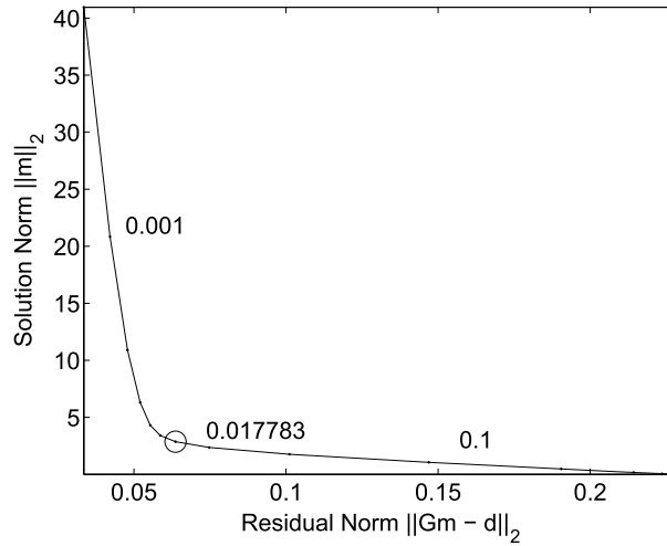
Figure 7.5 L-curve for zeroth-order Tikhonov solution with corner at \alpha = 0.01 .
