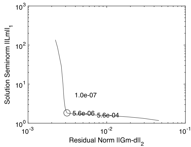
Figure 7.20 TV L-curve, with a corner at \alpha = 5.6 \times 10^{-6} .
