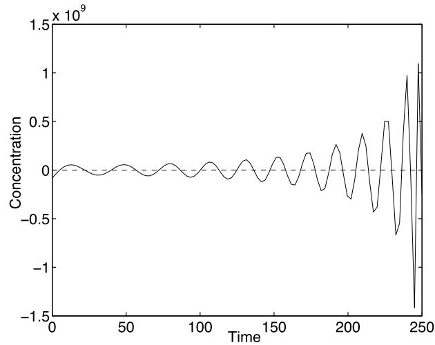
Figure 4.30 Least squares source history solution with true history (Fig. 4.28) shown as a dashed curve. Because the least squares solution has extremely large amplitudes, the true model appears as a flat line at this scale.
