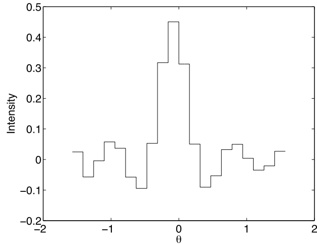
Figure 4.7 Resolution test using the spike model ( \alpha = 4.29 \times 10^{-5} determined from the discrepancy principle). Note that this model is nearly equivalent to that shown in Fig. 4.5.
