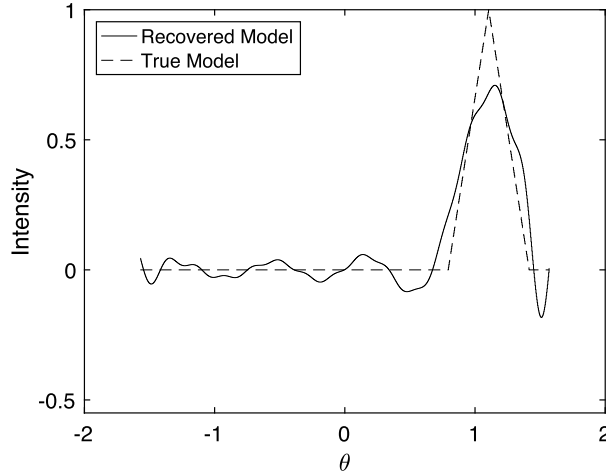
Figure 5.1 Recovery of a triangle function model with a width of 0.62 radians centered on \theta = 1.098 , satisfying the discrepancy principle using a set of 31 Fourier series model basis functions ( \alpha = 5.97 \times 10^{-6} , \chi = 4.48 \times 10^{-6} \approx \delta ).
