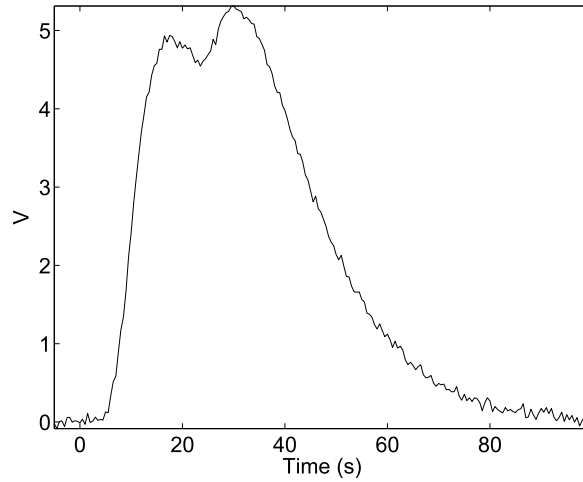
Figure 3.12 Predicted data from the true model plus independent N(0, (0.05)^2) (in units of volts) noise.
