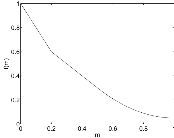
Figure 9.4 An example of a nonsmooth function.
