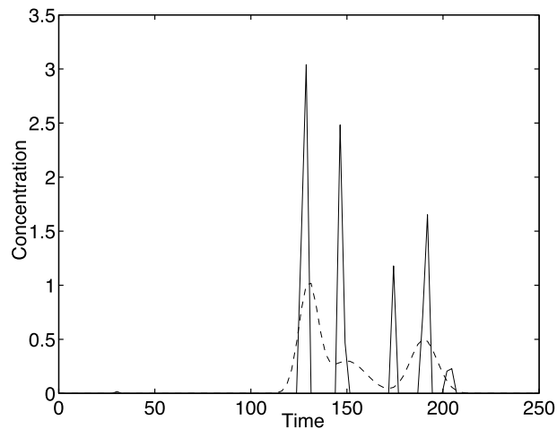
Figure 4.31 NNLS source history solution with true history (Fig. 4.28) shown as a dashed curve.
