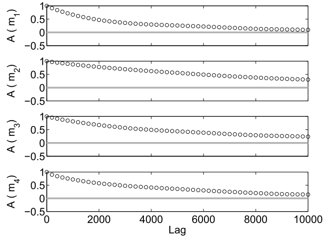
Figure 11.14 Autocorrelations for posterior distribution parameters prior to thinning for autocorrelation reduction.
