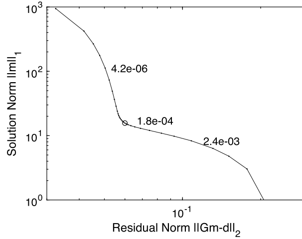
Figure 7.7 L-curve for the 1-norm regularized solution with corner near \alpha = 1.8 \times 10^{-4} .
