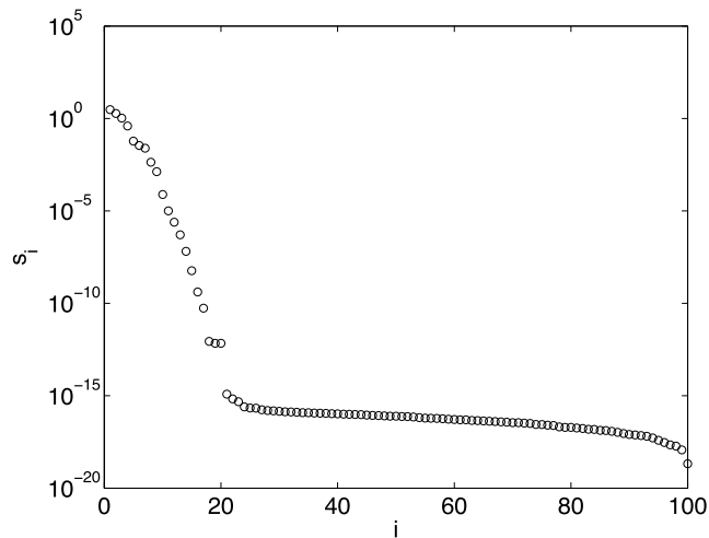
Figure 3.26 Singular values of \mathbf{G} for the Shaw example ( n = m = 100 ).
