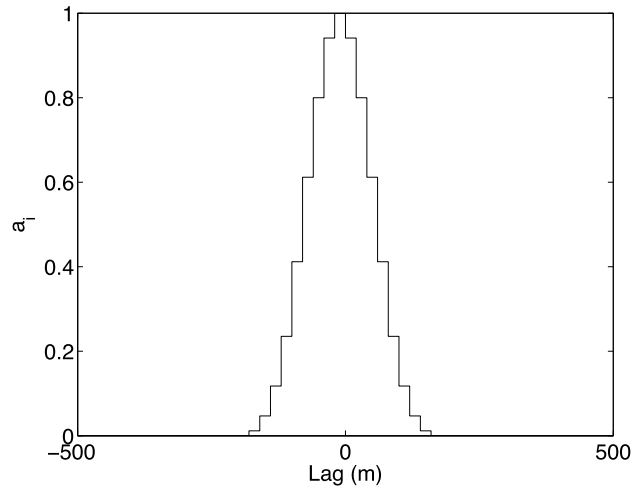
Figure 11.10 A correlation function for the prior distribution of Fig. 11.9 with a 1/e correlation length of approximately 5 parameters (100 m).
