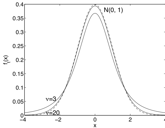
Figure B.3 The Student's t probability density function for \nu = 3 and \nu = 20 . Dashed curve shows the normal distribution N(0, 1) (Fig. B.2)
