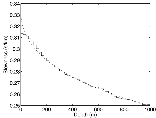
Figure 4.13 Tikhonov solution for the VSP problem, first-order regularization, \alpha = 122 , shown in comparison with the true model (Fig. 4.10).
