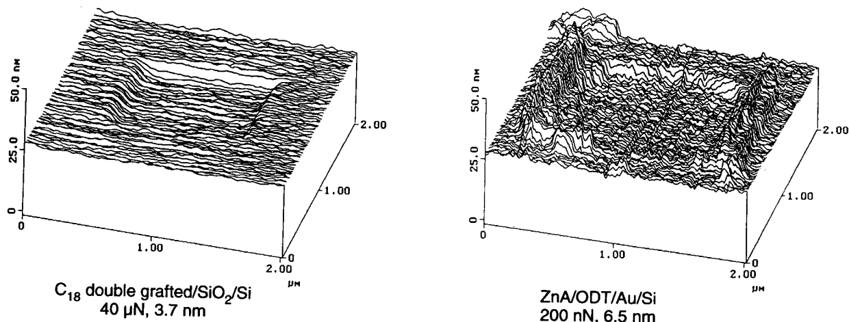
FIG. 5 Surface profiles showing the worn region after one scan cycle for self-assembled monolayers of octadecyl silanol (left) and zinc arachidate (right). Normal force and the wear depths are indicated. Note
