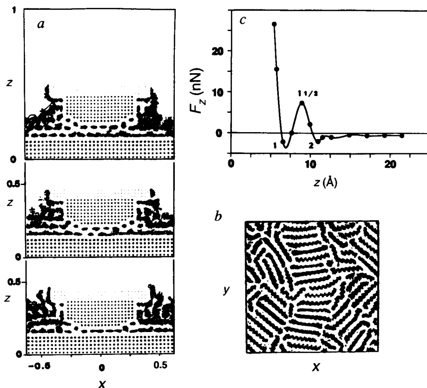
FIG. 7 a , Side views of atomic configurations of a nickel tip, an Au(001) surface and an n\text{-C}_{16}\text{H}_{34} (hexadecane) film, starting at a tip-to-surface spacing corresponding to two layers of the confined film ( d_{ts} = 11 Å, top) and ending with a one-layer film ( d_{ts} = 6.5 Å, bottom). The middle configuration corresponds to spacing d_{ts} = 9 Å. The linear dimension of the system along the x axis is 77.5 Å, and the configurations were obtained in a vertical slice in the xz plane of a width of 16 Å. In this figure, the coordinate axes are normalized such that x = z = 1 corresponds to a linear dimension of 77.5 Å. b , Short-time trajectories of hexadecane molecules in the layer next to the Au(001) surface, corresponding to the one-layer confined film shown at the bottom of a , illustrating intra-layer ordered domains. (The linear dimension of the system along the x and y axes is 77.5 Å.) c , Normal force on the nickel tip versus the distance between the tip and the gold surface, z , recorded during the process of lowering of the nickel tip onto the hexadecane-covered Au(001) surface, and illustrating force oscillations associated with the layering transformations in the film.
