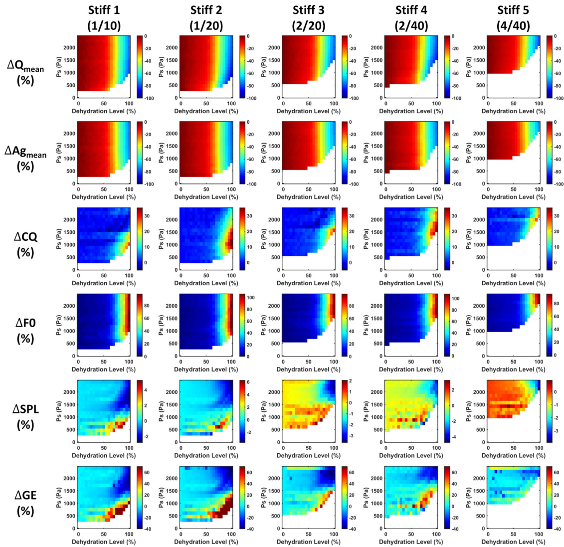
FIGURE 5. Percentage changes of the mean glottal flow rate \Delta Q_{\text{mean}} , mean glottal area \Delta A_{\text{g,mean}} , closed quotient \Delta CQ , fundamental frequency \Delta F0 , sound pressure level \Delta SPL , and glottal efficiency \Delta GE with the increasing dehydration levels under different vocal fold stiffness conditions. For all cases, the dehydration distribution is uniform. The values in the parentheses represent the transverse Young’s modulus E_t and AP shear modulus G_{ap} of the vocal fold. AP, anterior-posterior.
